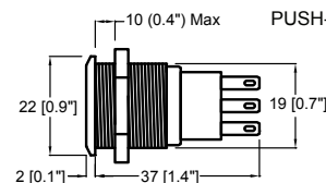
PUSH-BUTTON SWITCHES
