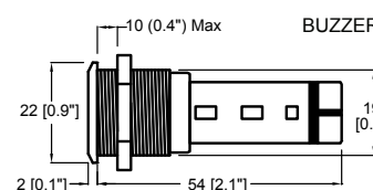
BUZZER UNITS
