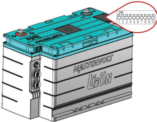
Figure 9: DIP switches
